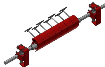
REMACLEAN HM-U8
