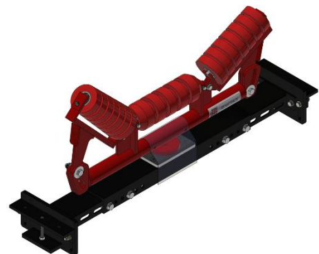
REMATRACK OT
