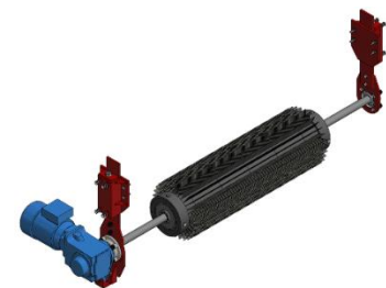
REMACLEAN GBM
