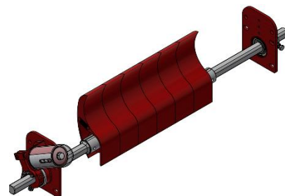
REMACLEAN PUR-F5
