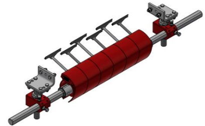
REMACLEAN HM-U7
