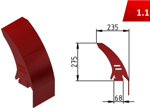
Segment PUR-F7
