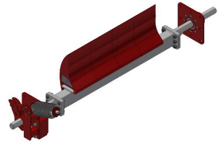
REMACLEAN PUR-F300
