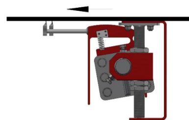
Einbau REMACLEAN HM-U500
