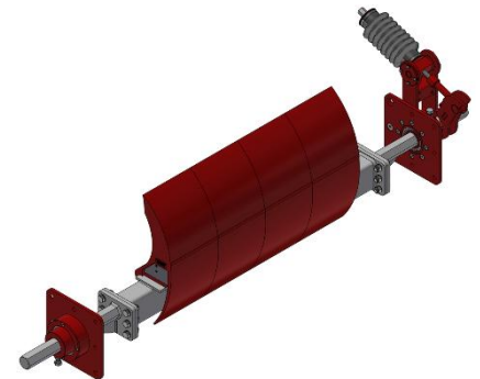
REMACLEAN PUR-F400
