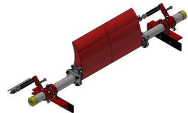
REMACLEAN PUR-F4
