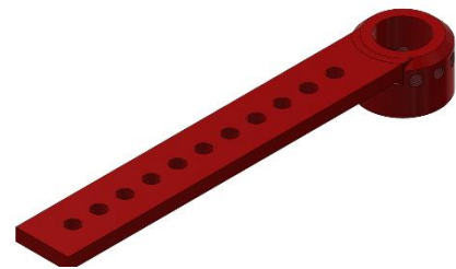
Verstellarm HM-U7/U8
