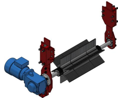
REMACLEAN SGB
