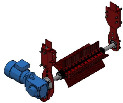
REMACLEAN SGB-PUR
