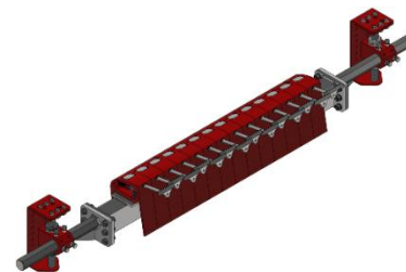
REMACLEAN HM-U500
