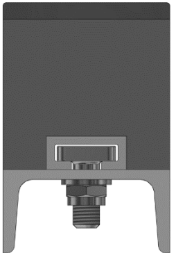
REMASLIDE V
